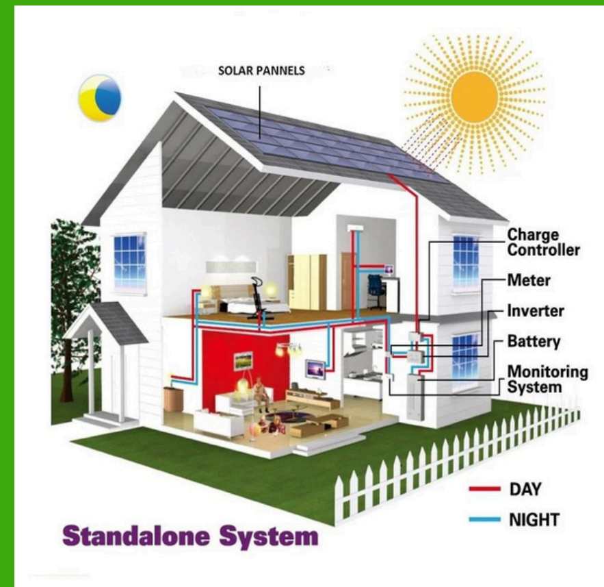
Off Grid Solar System
